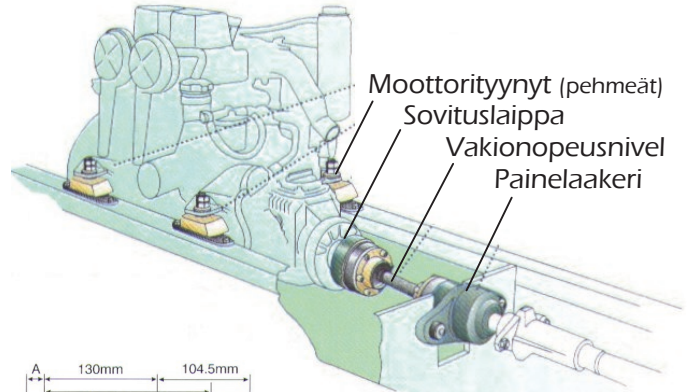
Aquadrive CVB 05.10 esim. 45 hv/3800rpm, välitys 2:1, max 4000rpm A (Adapterilaiippa) ~25mm
