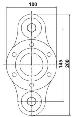
Aquadrive CVB 05.10 esim. 45 hv/3800rpm, välitys 2:1, max 4000rpm A (Adapterilaiippa) ~25mm
