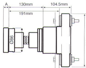
Aquadrive CVB 05.10 esim. 45 hv/3800rpm, välitys 2:1, max 4000rpm A (Adapterilaiippa) ~25mm
